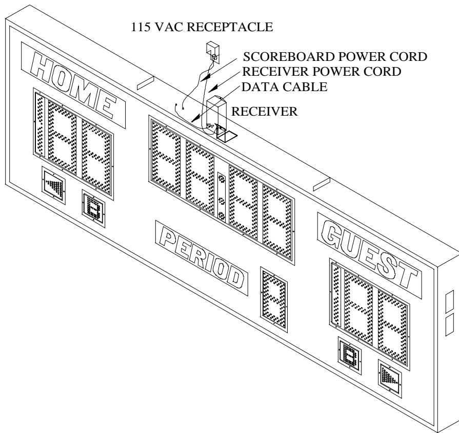
Figure 3 SCORELINK 200 Receiver Installation
