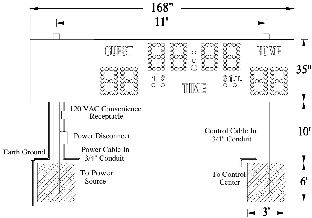
Figure 2 MP-9450 with Optional Side Sponsor Panel Post Spacing
