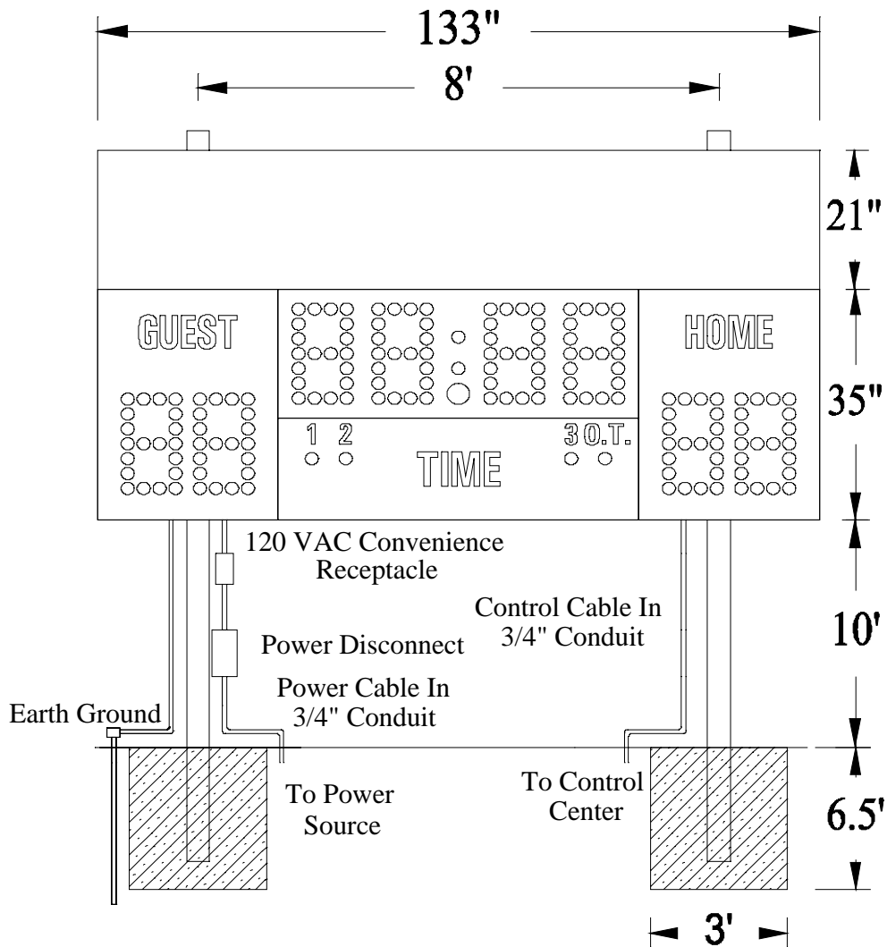
Figure 3 MP-9450 with Optional Top Sponsor Panel Post Spacing
