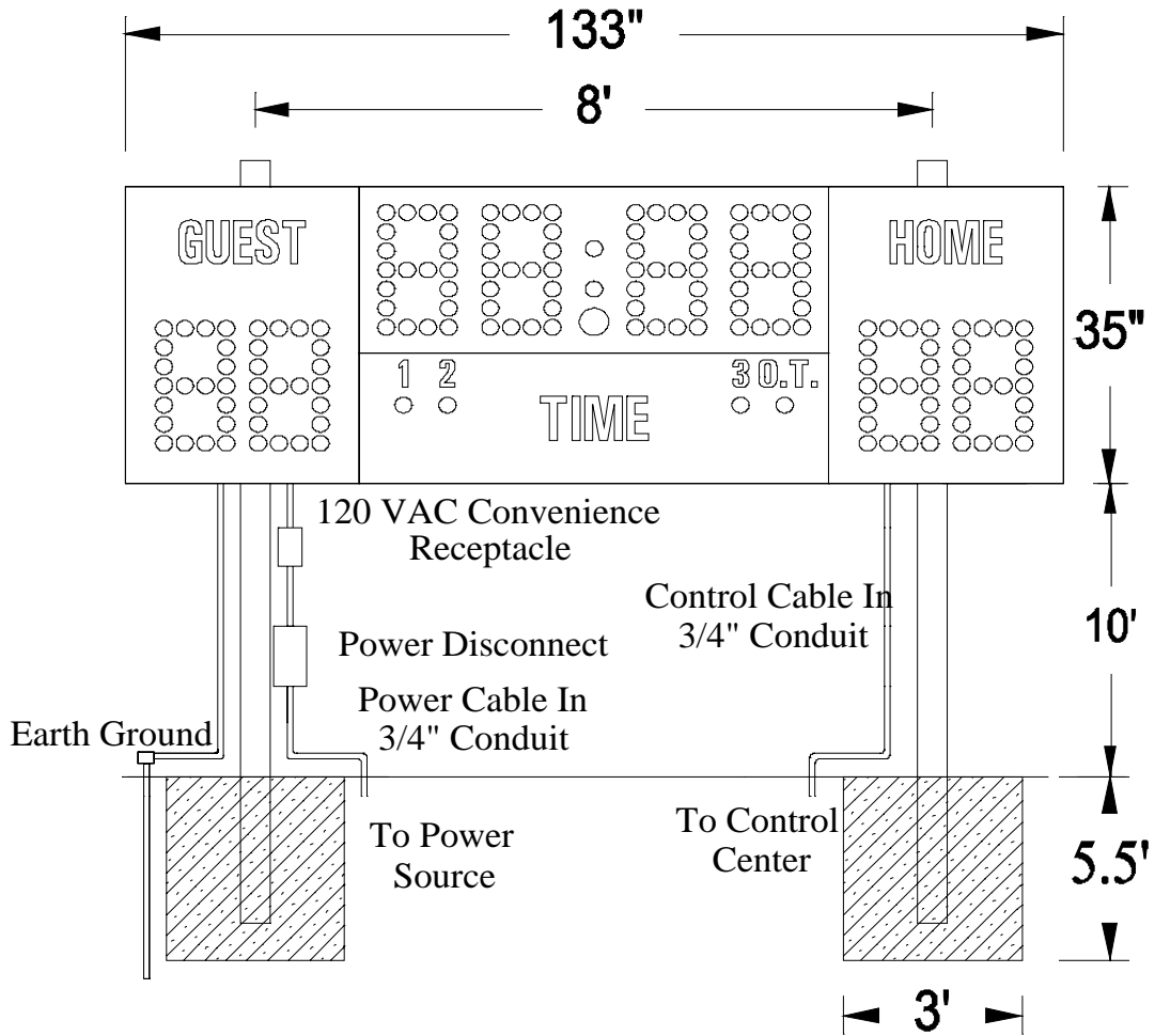
Figure 1 MP-9450 Post Spacing
