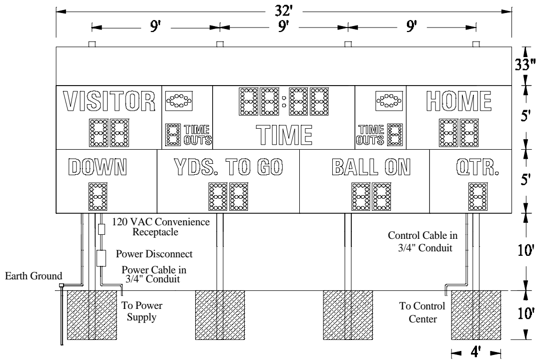
Figure 2 MP-375 with Optional Top Sponsor Panel Post Spacing
