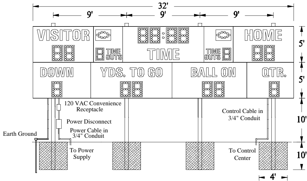
Figure 1 MP-375 Post Spacing
