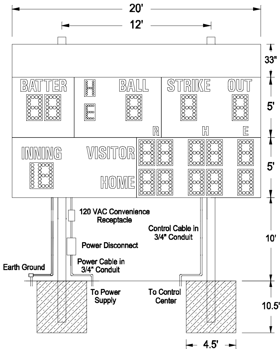
Figure 2 MP-140 with Optional Top Sponsor Panel
