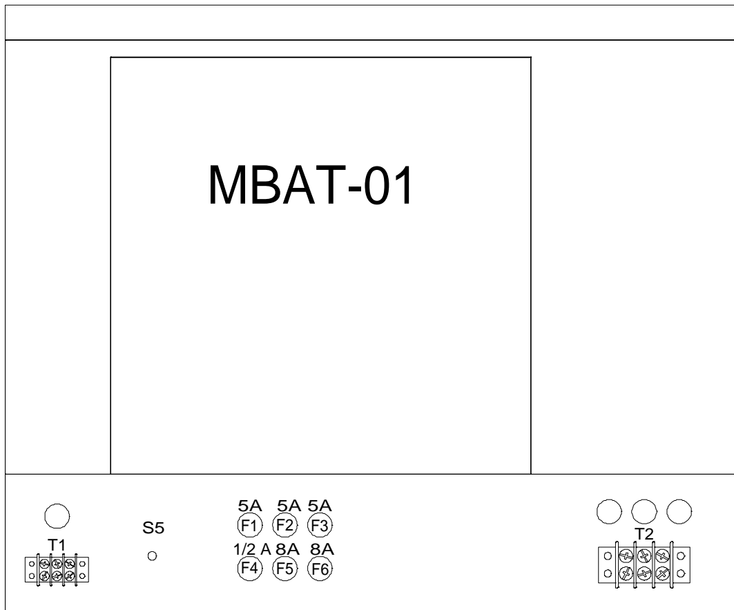
Figure 9 Upper Access Panel Removed
