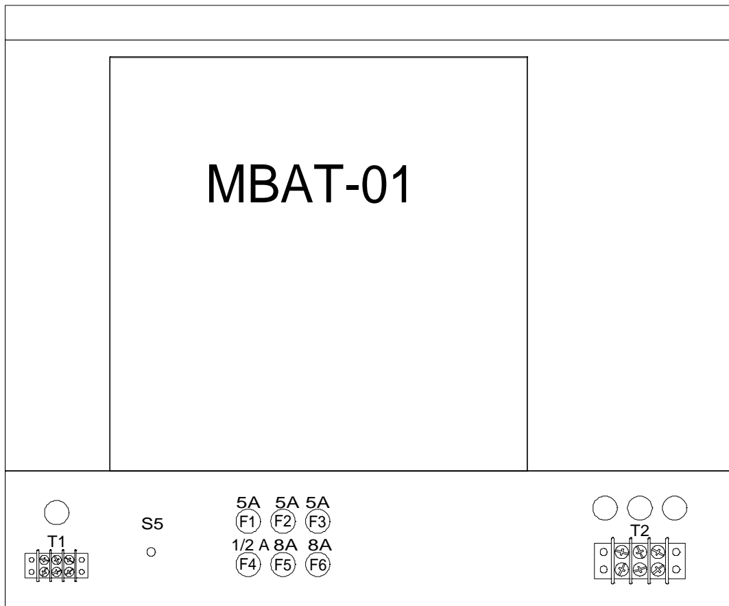
Figure 13 Upper Access Panel Components
