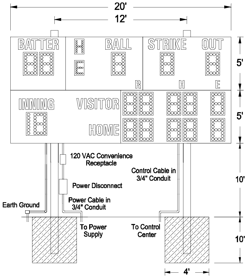
Figure 1 MP-140 Post Spacing
