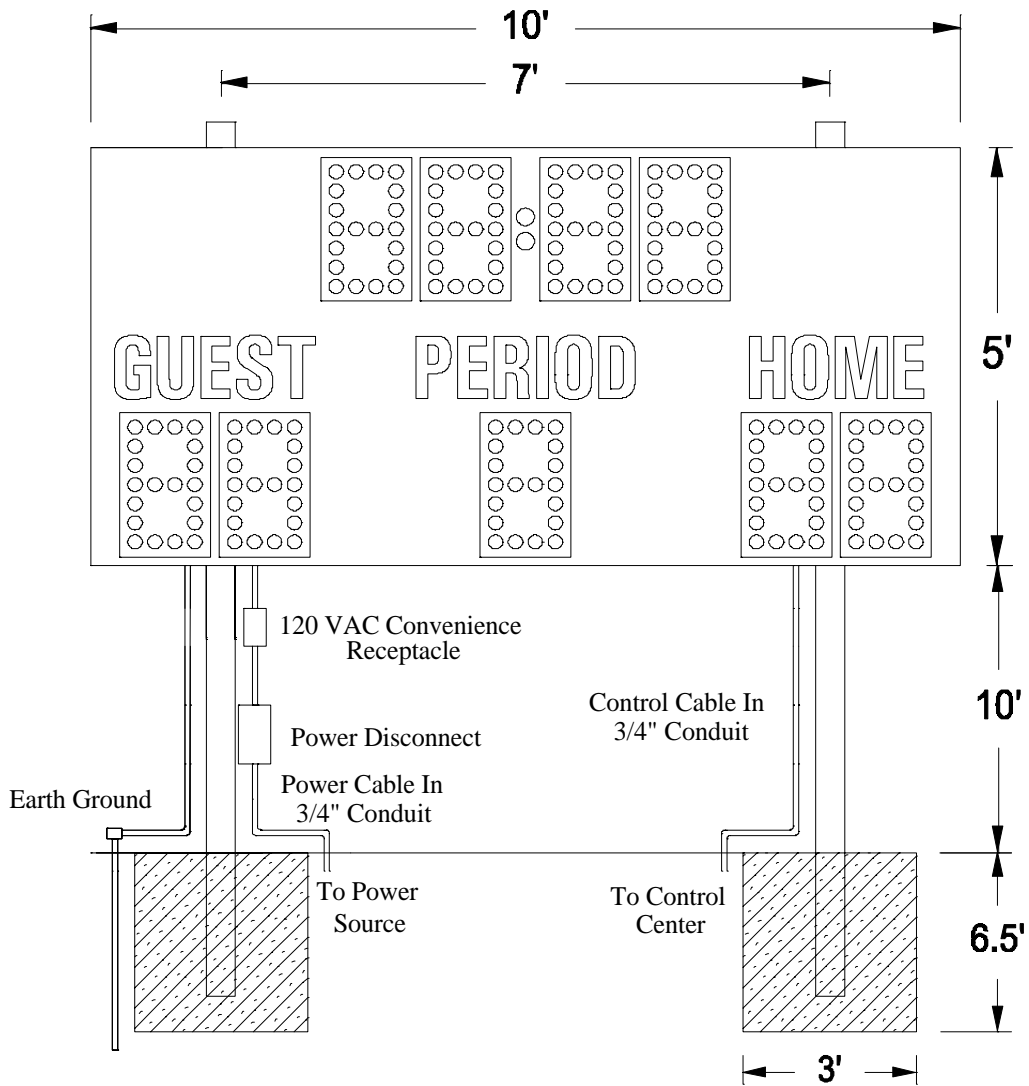
Figure 1 MM-365 Post Spacing
