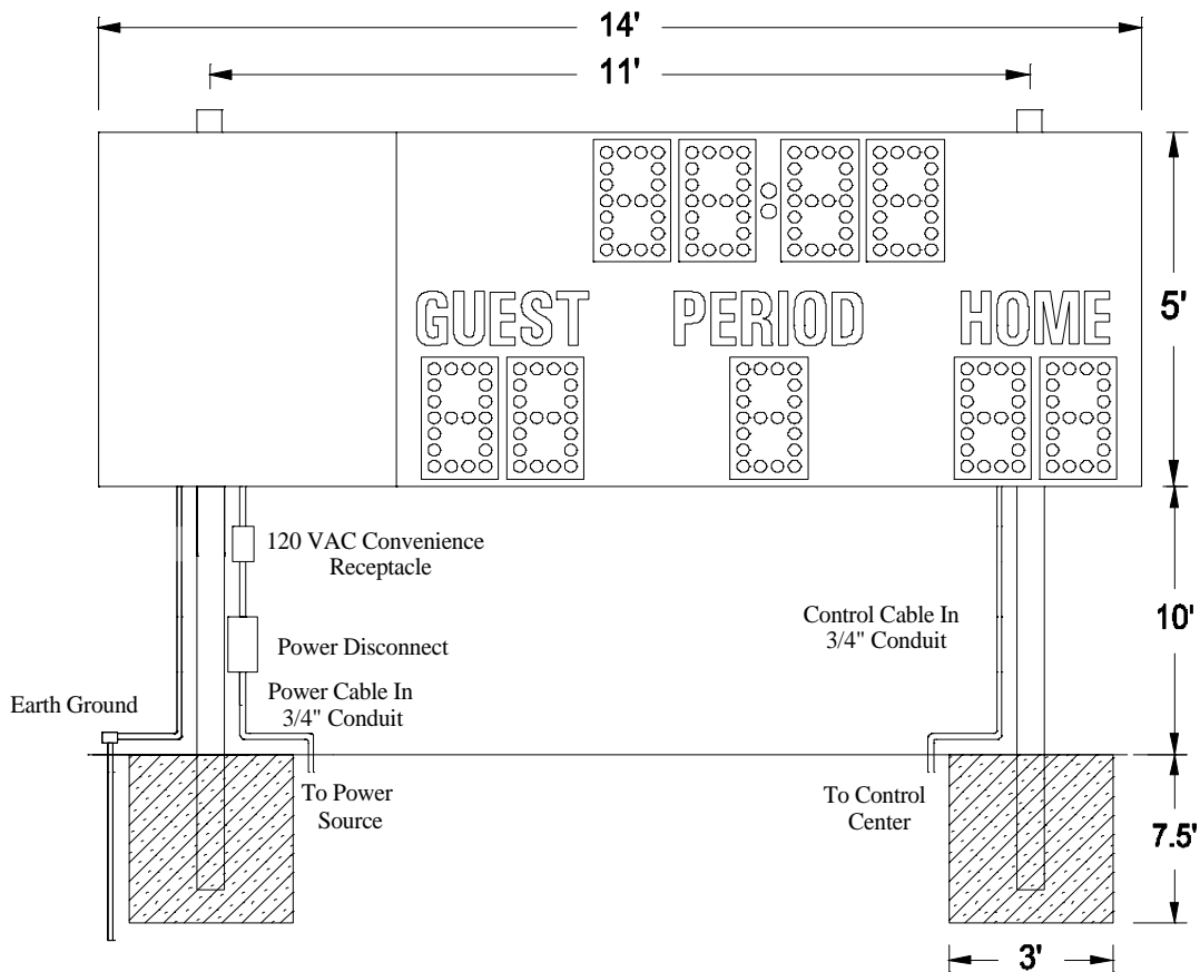
Figure 3 MM-365 with Optional Side Sponsor Panel Post Spacing
