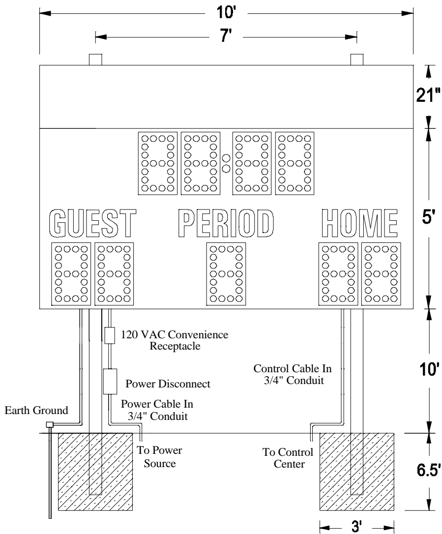
Figure 2 MM-365 with Optional Top Sponsor Panel Post Spacing
