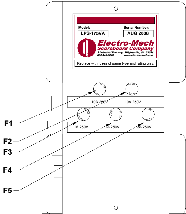
Figure 9 LPS-175VA POWER SUPPLY MODULE
