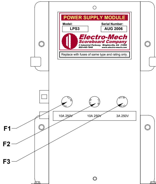
Figure 10 LPS3 POWER SUPPLY MODULE
