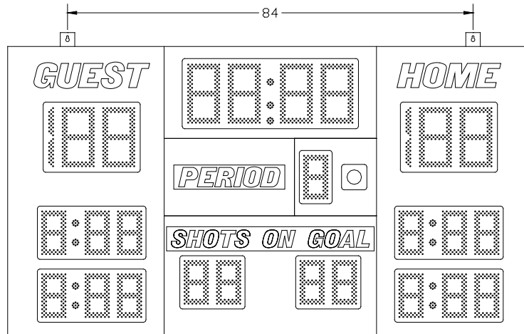
Figure 1 Model 8750 Mounting Points
