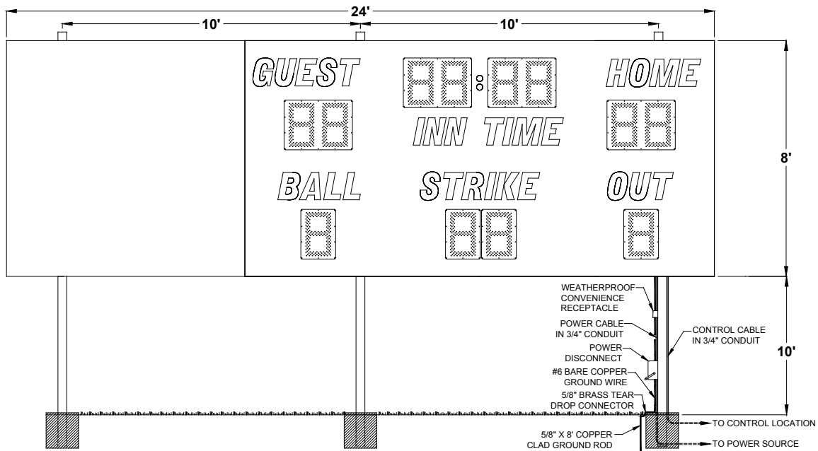
Figure 2 3450 with Optional Side Sponsor Panel Post Spacing
