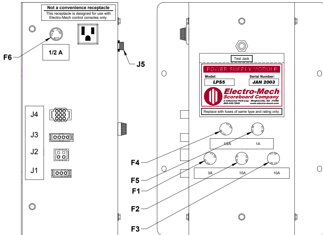
Figure 22 LPS5 Fuse Locations
