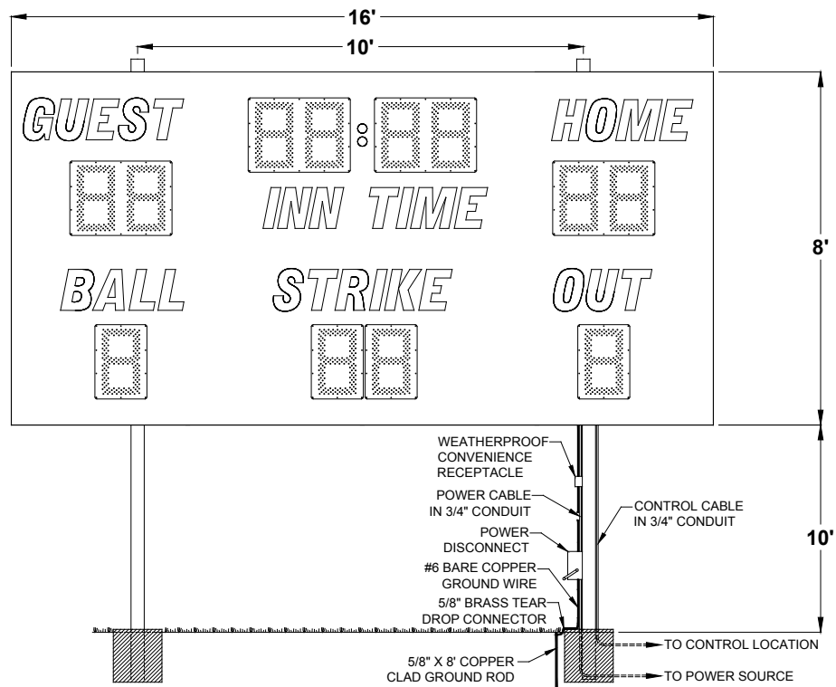
Figure 1 3450 Post Spacing
