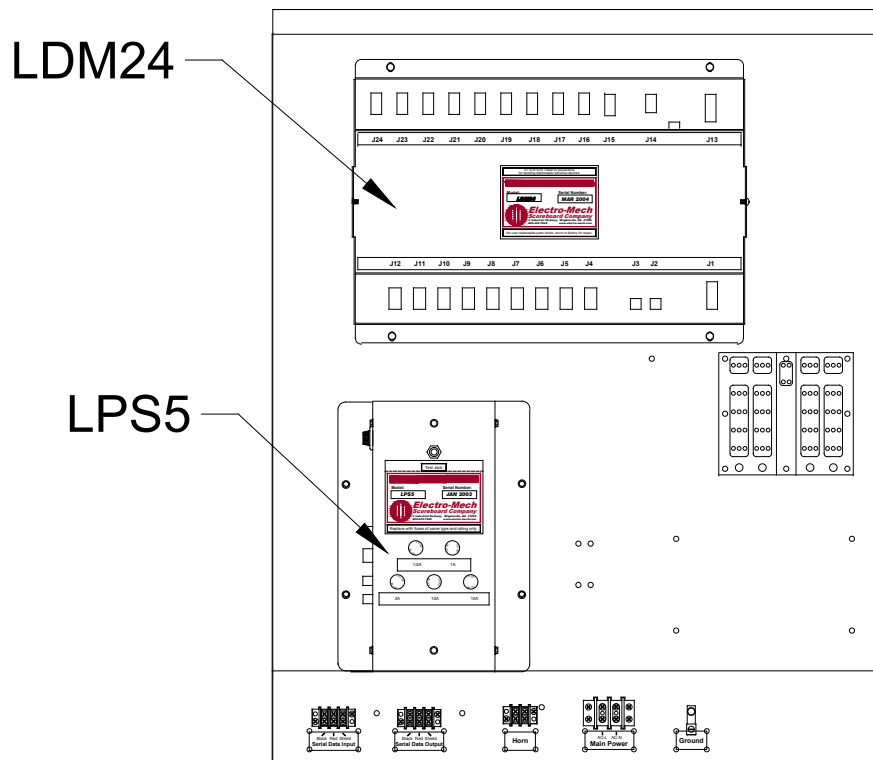
Figure 7 Access Panel Removed
