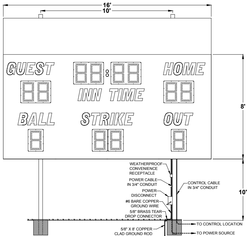
Figure 3 3450 with Top Sponsor Panel Post Spacing
