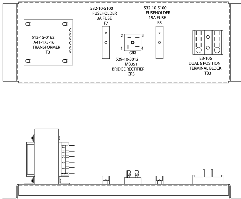
Figure 13 Stat Panel Section Power System
