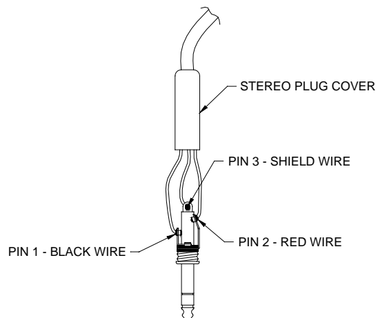
Figure 4 1/4-inch Stereo Plug Wiring Diagram
