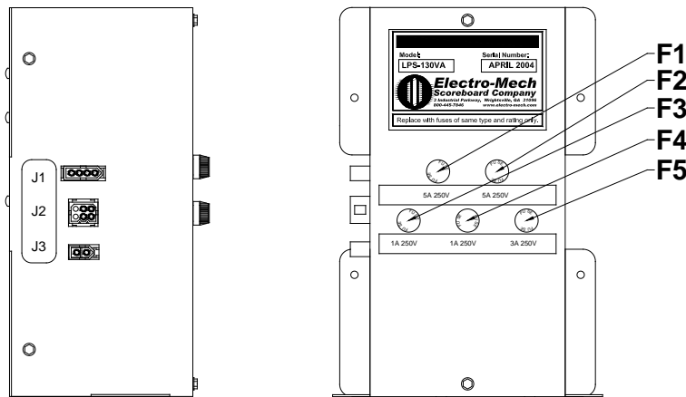
Figure 12 LPS-130VA Power Supply Module
