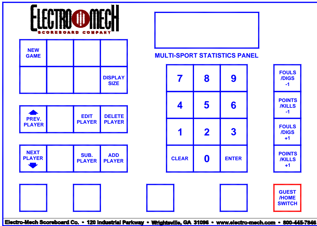
Figure 7 2056 Keypad Layout
