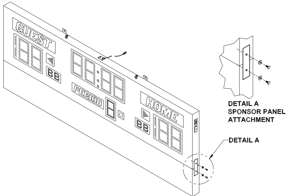
Figure 2 2370 with Bottom Sponsor Panel Attached
