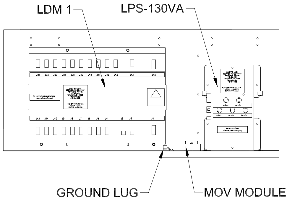
Figure 10 SCOREBOARD ELECTRONICS
