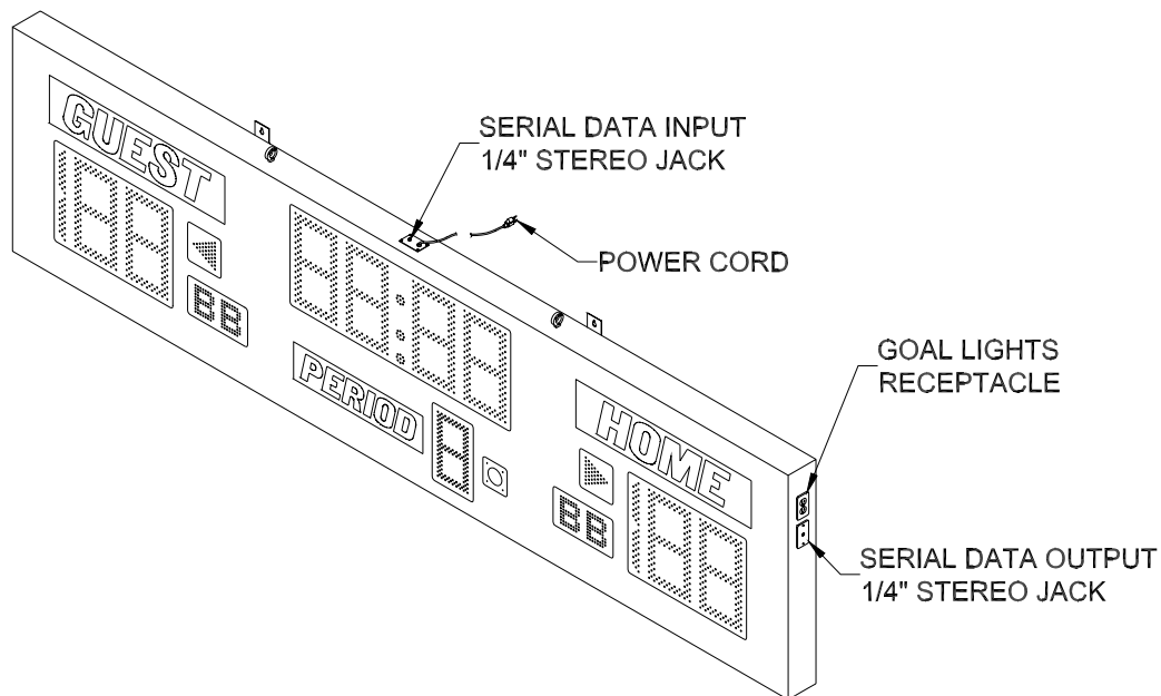
Figure 3 Electrical Connection Points
