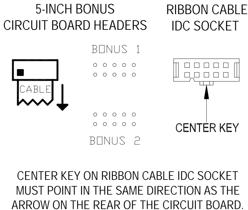
Figure 9 BONUS 1 and BONUS 2 Ribbon Cable Connection Diagram
