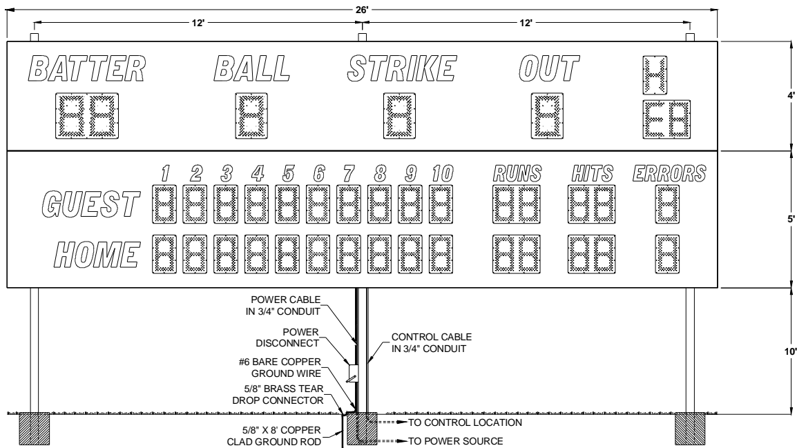
Figure 1 1550 Post Spacing
