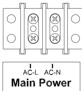
Figure 9 Power to Scoreboard Connections
