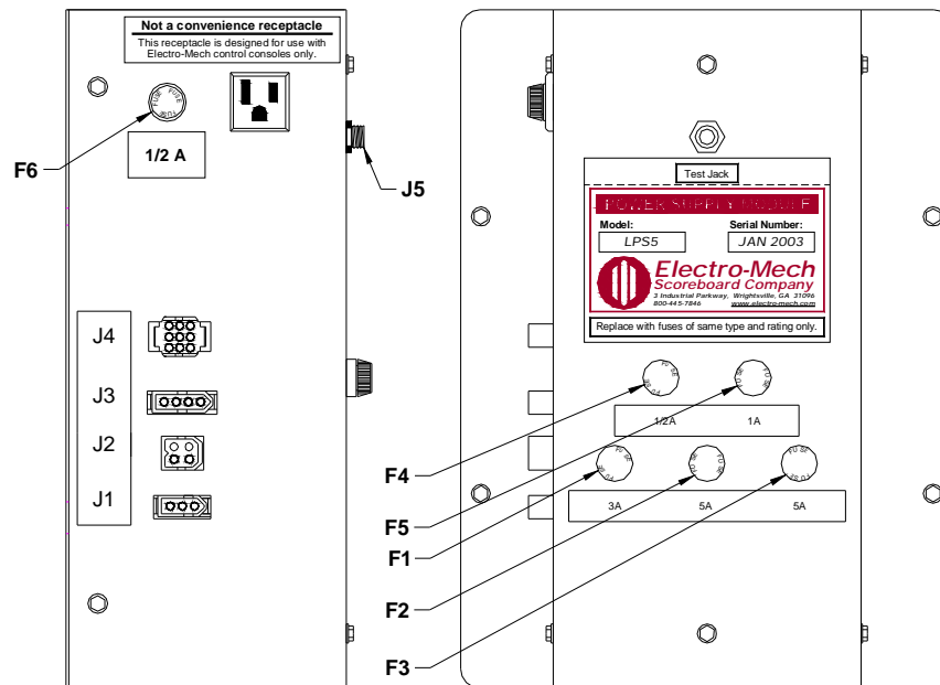
Figure 18 LPS5 Fuse Locations
