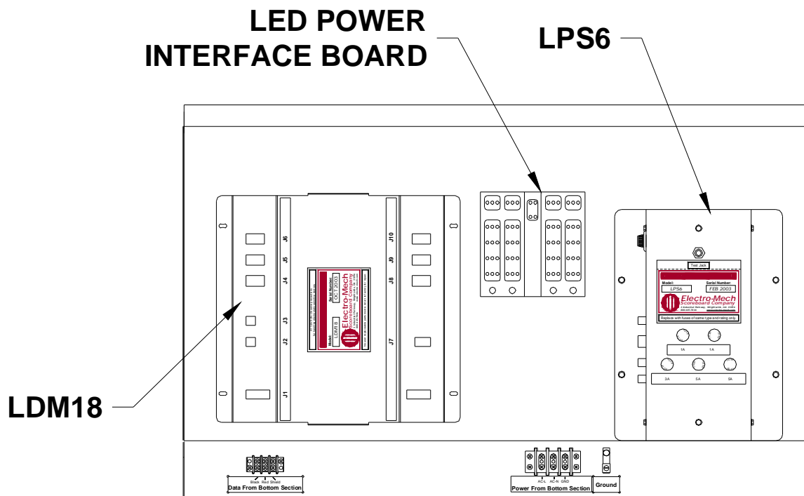
Figure 20 Upper Access Panel Components
