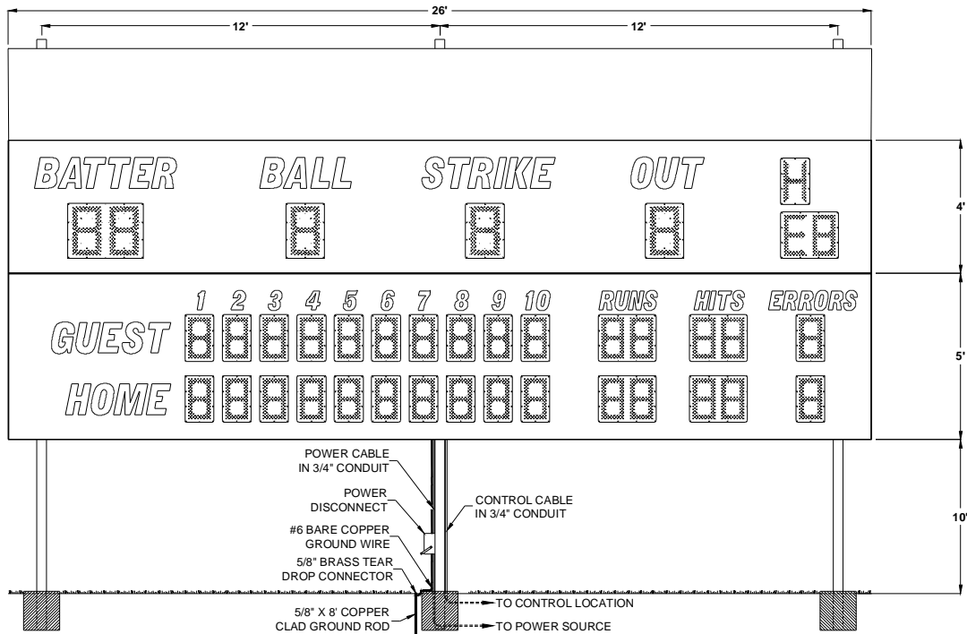
Figure 2 1550 with Optional Top Sponsor Panel Post Spacing
