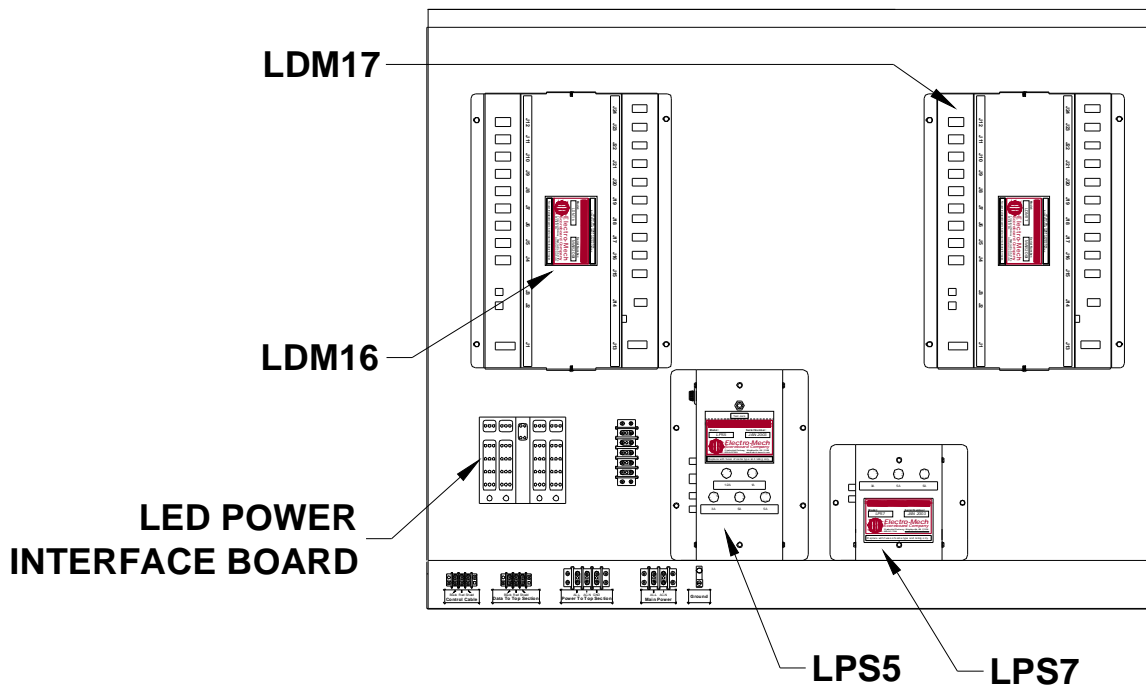
Figure 17 Lower Access Panel Components
