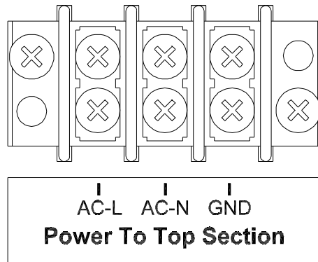
Figure 7 Power to Top Section Connections
