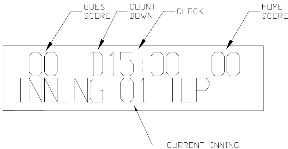
Figure 13 Control Console LCD Display
