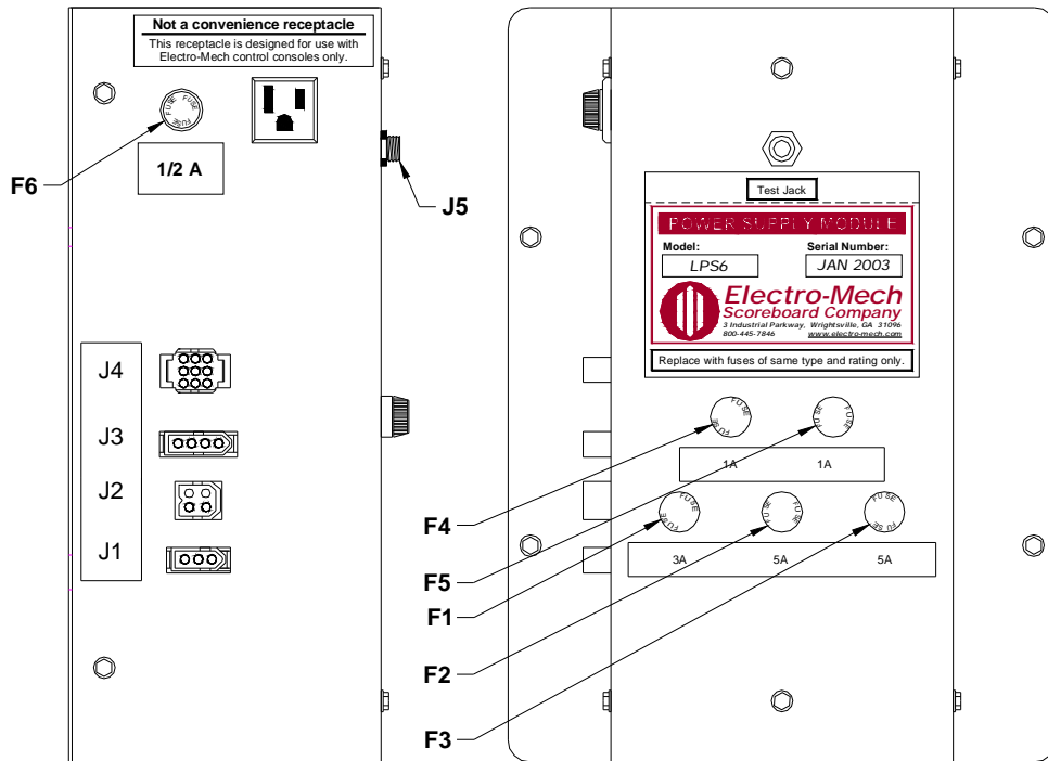
Figure 21 LPS6 Fuse Locations
