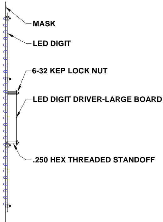
Figure 16 LED Digit Driver - Large Board
