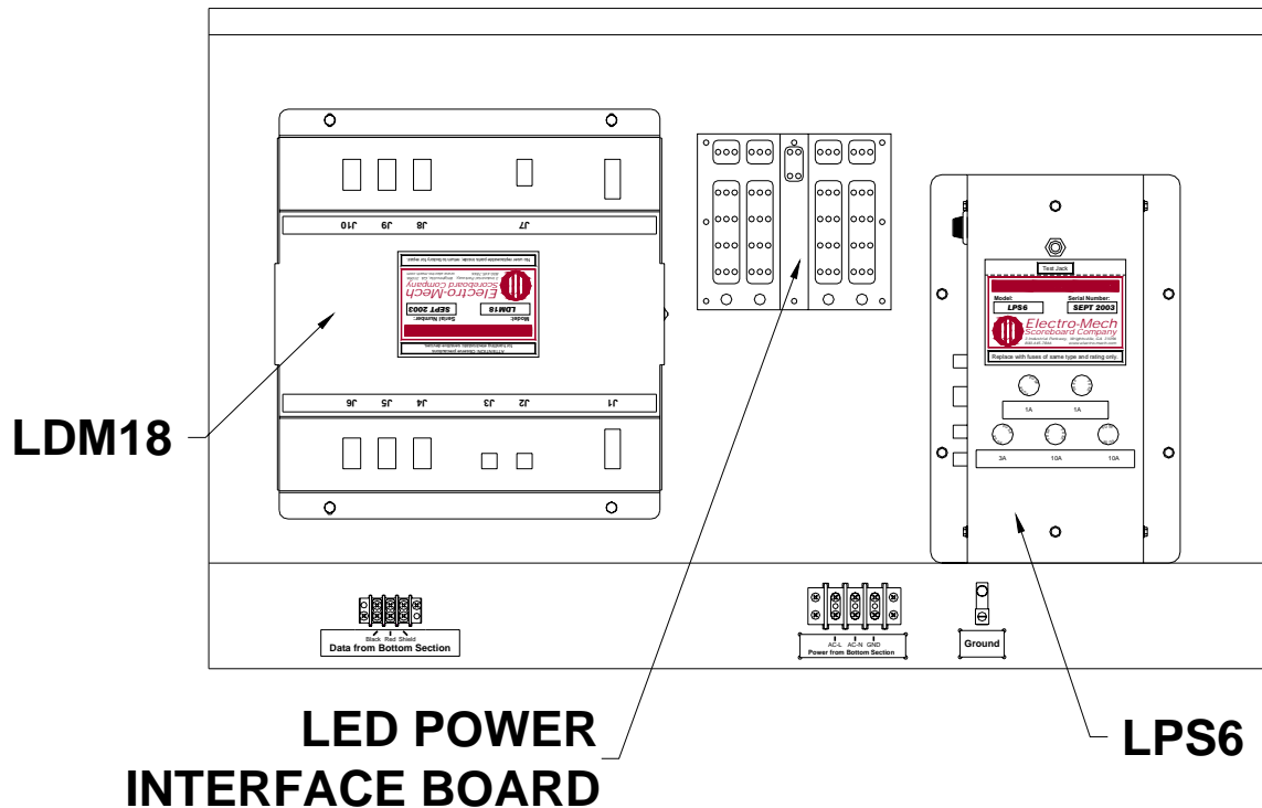
Figure 17 Upper Access Panel Components
