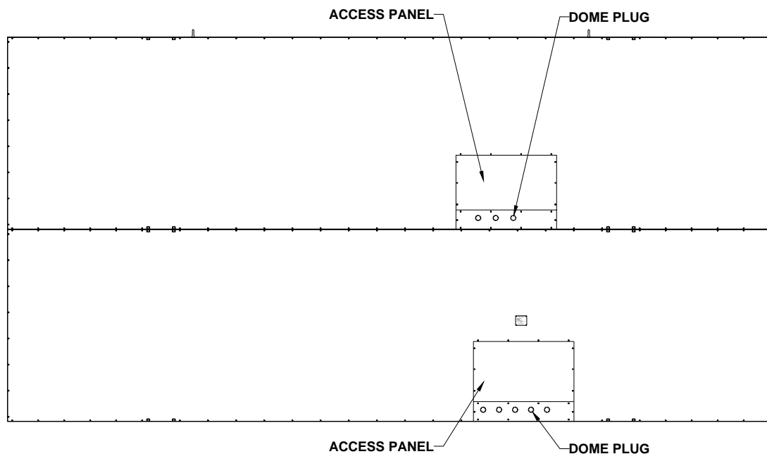
Figure 5 Rear Access Panels
