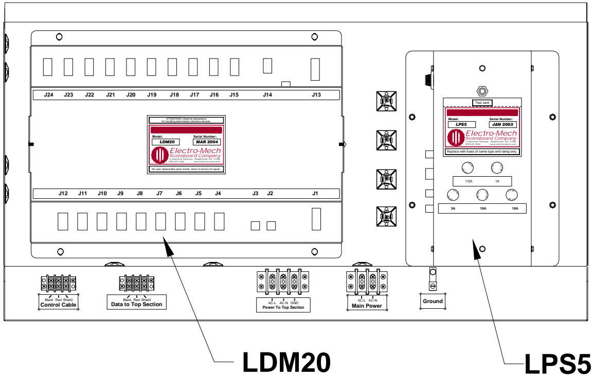
Figure 15 Lower Access Panel Components
