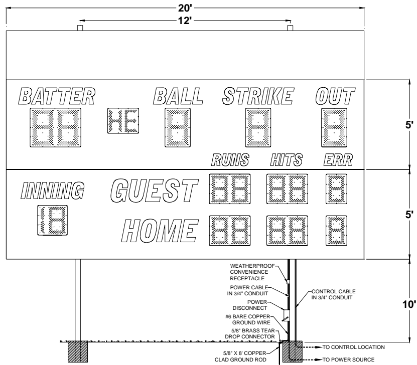
Figure 2 1480 with Optional Top Sponsor Panel Post Spacing
