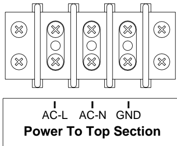
Figure 6 Power to Top Section Connections
