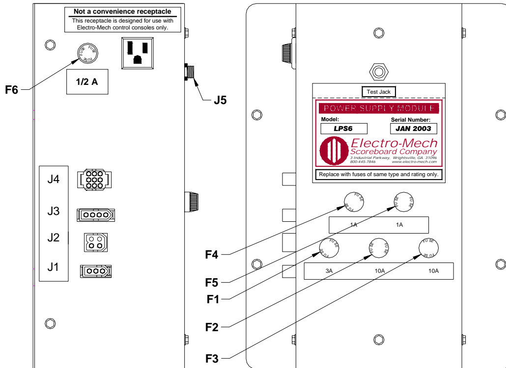
Figure 18 LPS6 Fuse Locations
