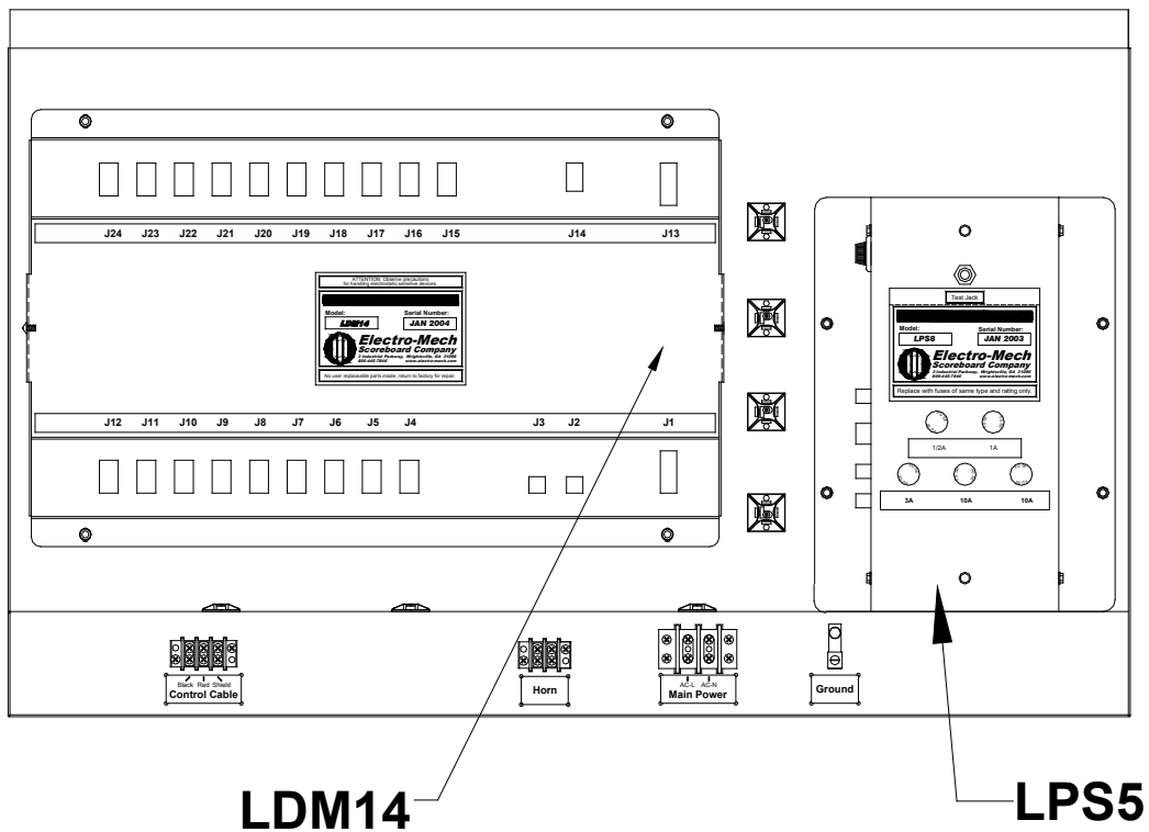
Figure 7 Access Panel Removed
