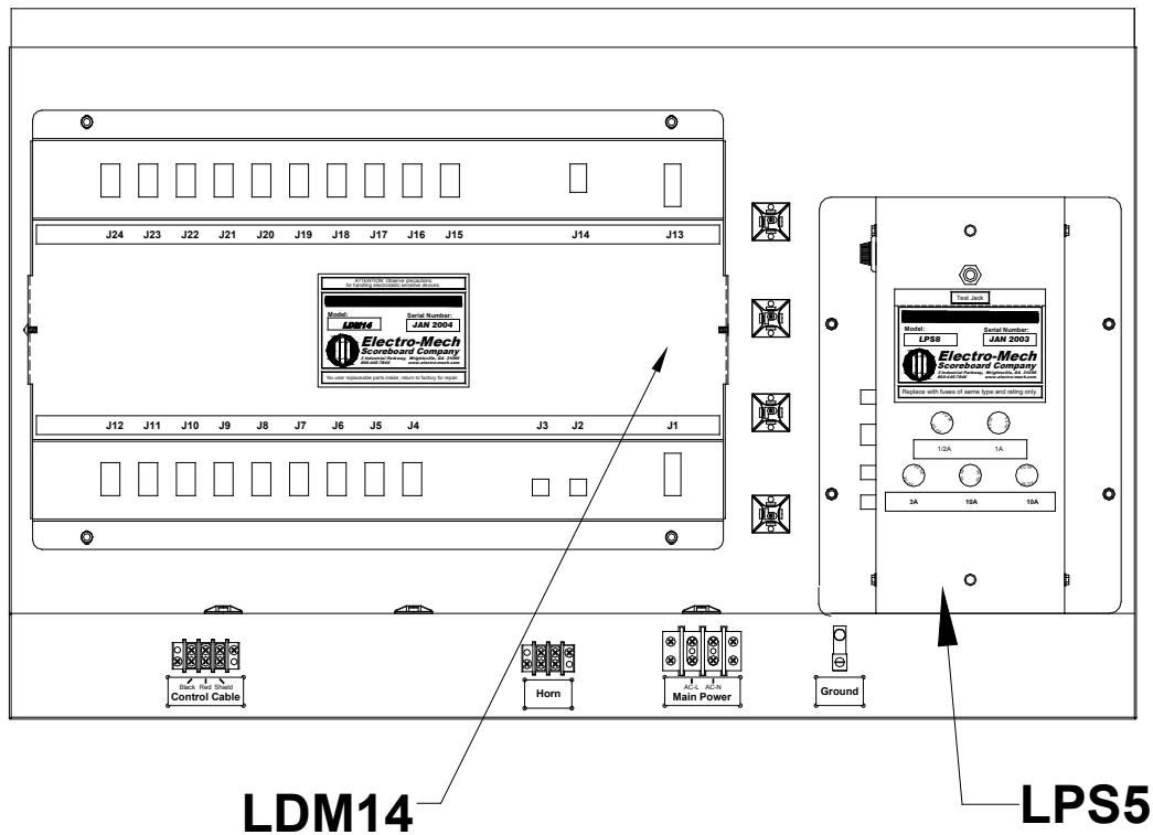
Figure 15 Access Panel Components
