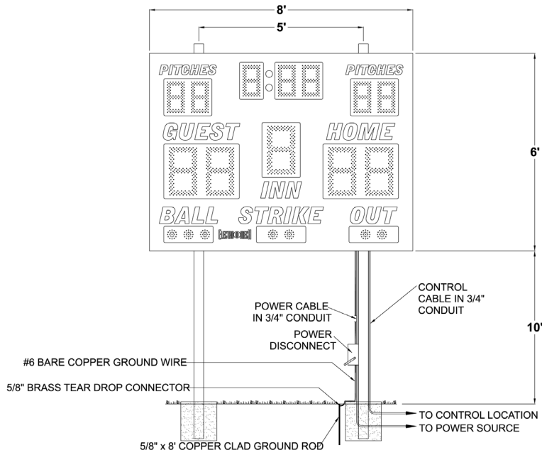
Figure 1 Model 1131 Post Spacing
