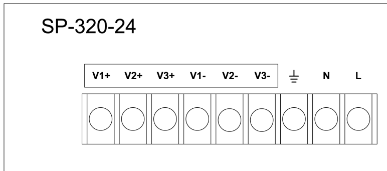
Figure 14 Power Module Screw Terminals
