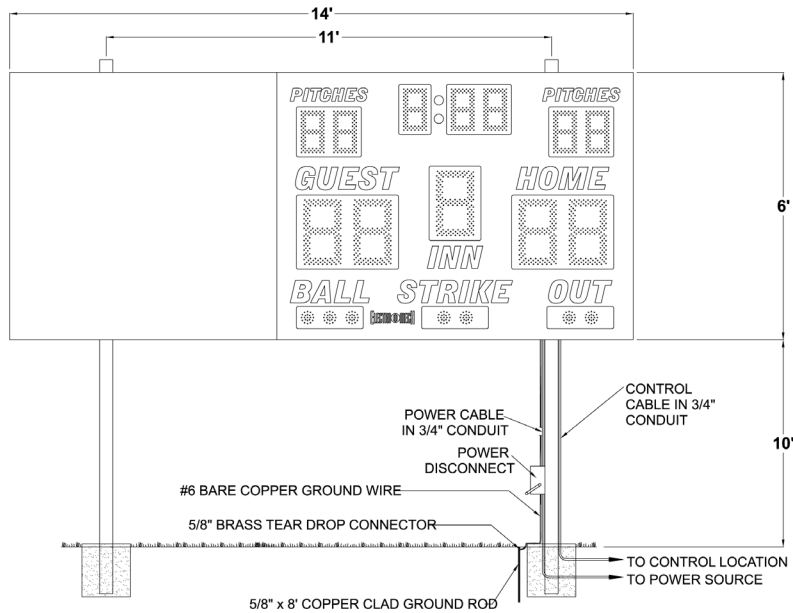
Figure 2 Model 1131 with Side ID Panel Post Spacing
