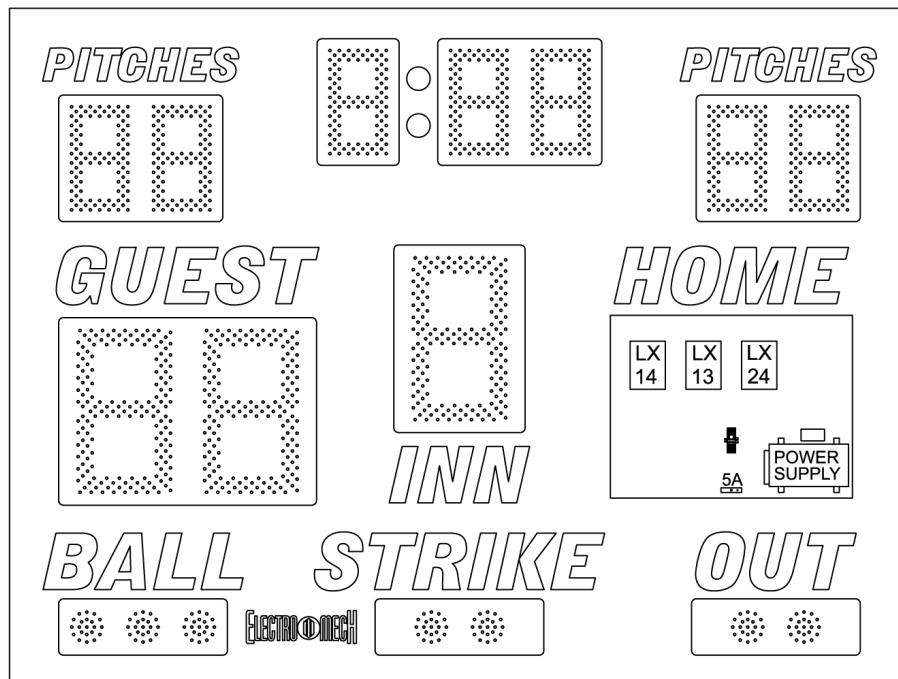
Figure 13 Component Locations
