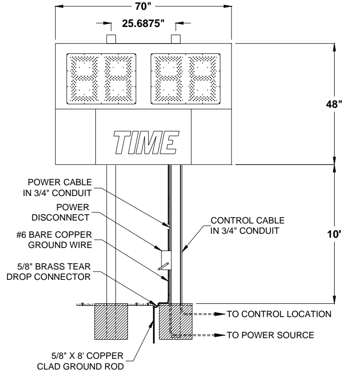
Figure 1 1064 Post Spacing
