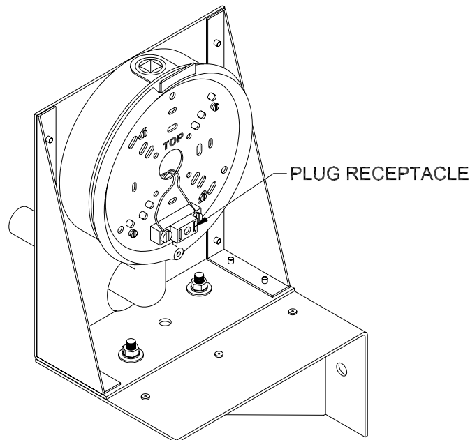
Figure 9 Plug Receptacle Wire Attachment
