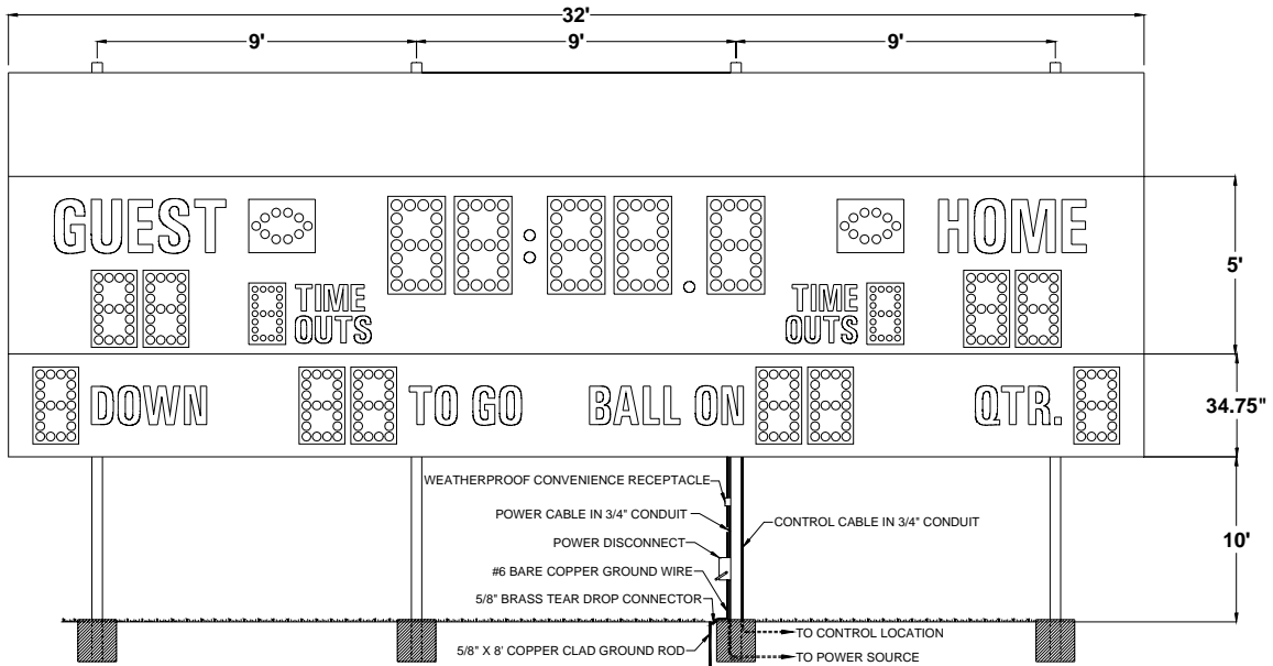
Figure 2 MP-374-TK with Top Sponsor Panel Post Spacing
