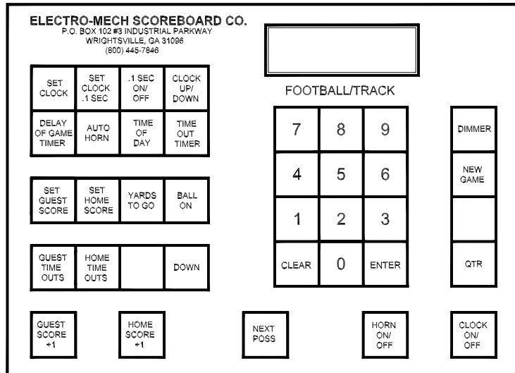
Figure 20 Keypad Layout
