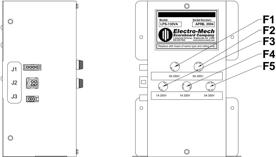
Figure 13 LPS-130VA POWER SUPPLY MODULE
