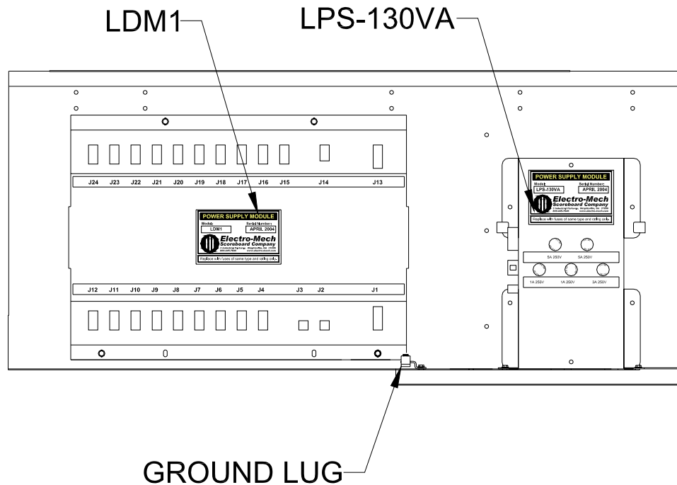
Figure 12 Scoreboard Electronics
