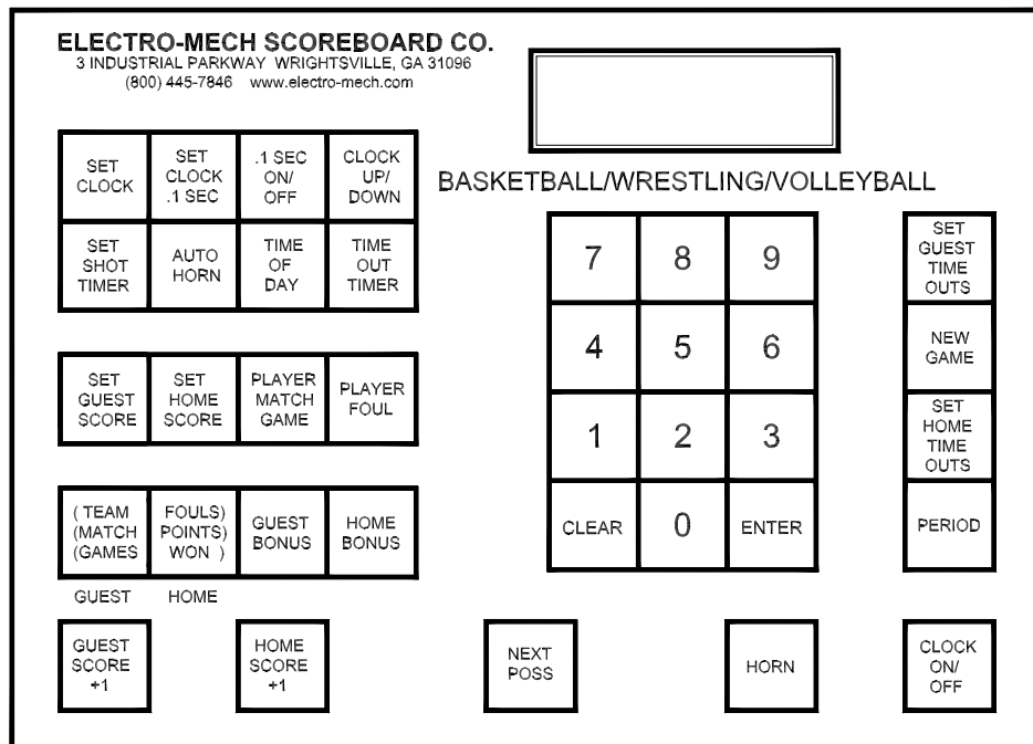
Figure 7 2570 Keypad Layout
