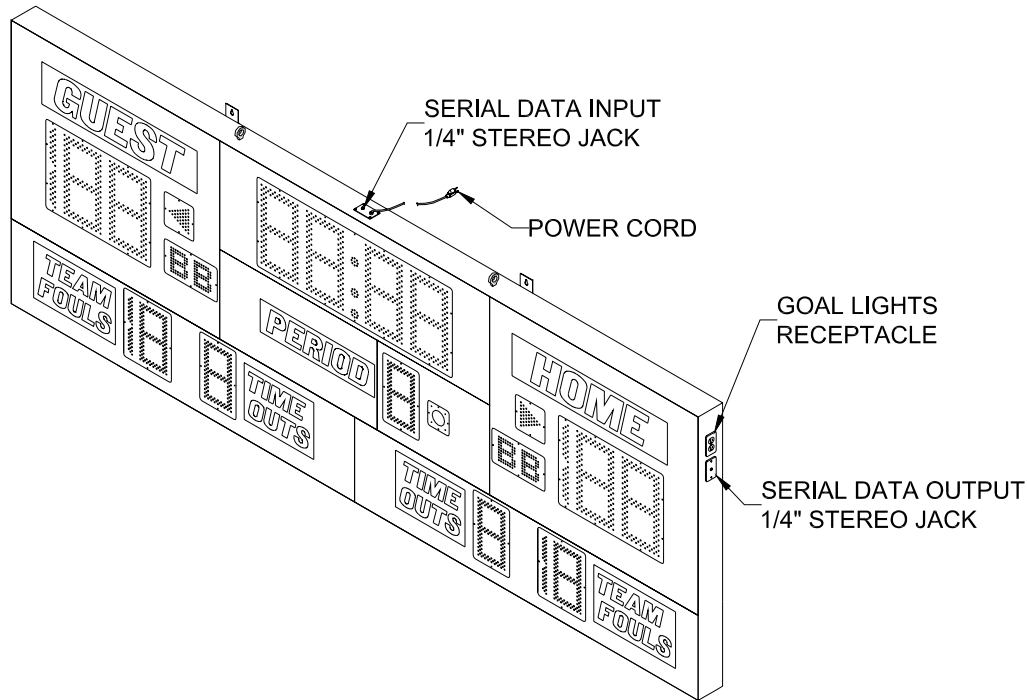
Figure 4 Electrical Connection Points
