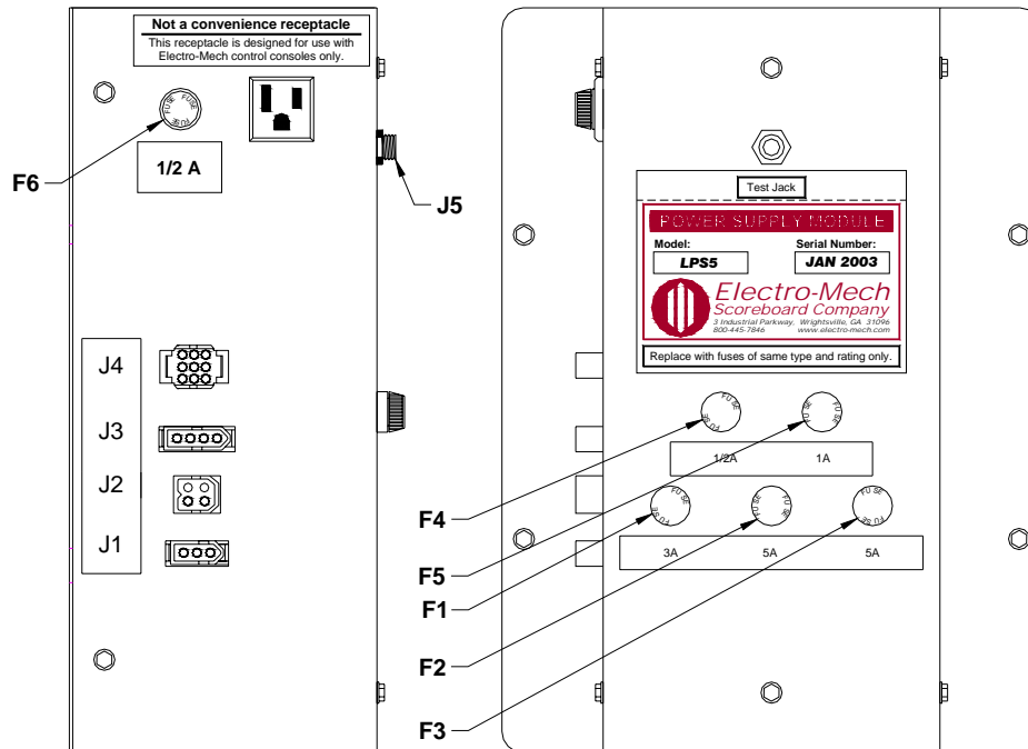
Figure 18 LPS5 Fuse Locations
