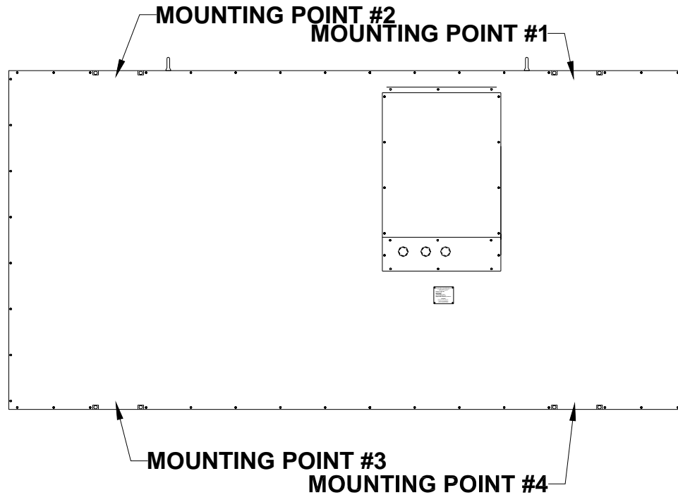
Figure 4 Mounting Points
