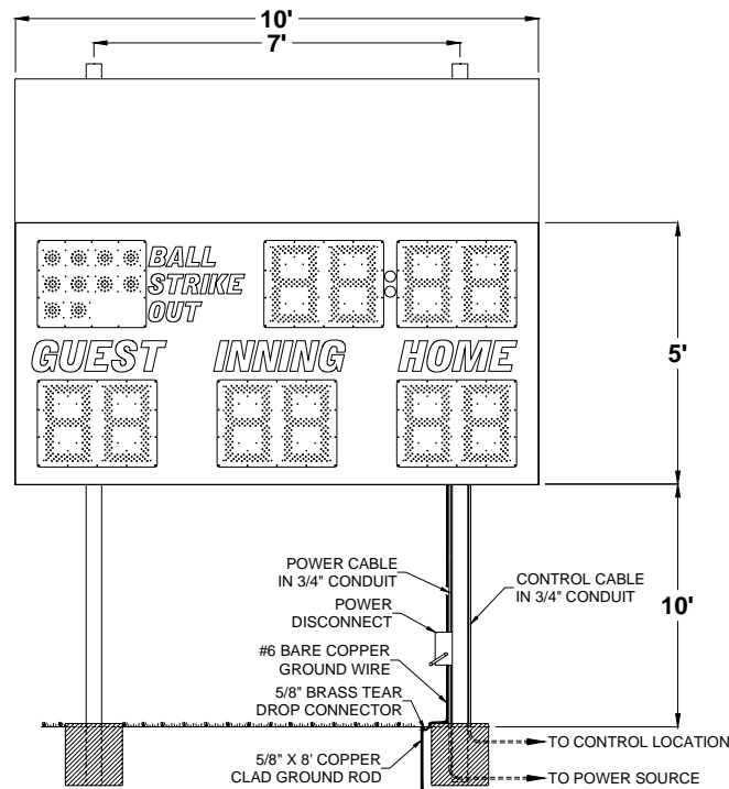
Figure 3 1360 with Top Sponsor Panel Post Spacing
